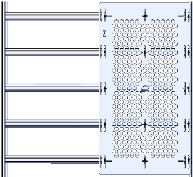
Layout 2: Using 14 M8 Bolts & Channel Nuts
