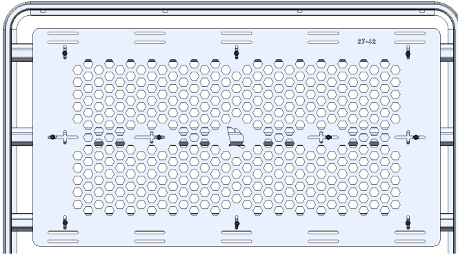
Layout 2: Using 14 M8 Bolts & Channel Nuts
